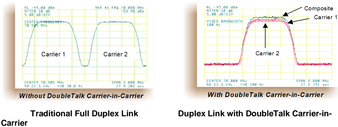
Figure 3-13. Duplex Link Optimization
