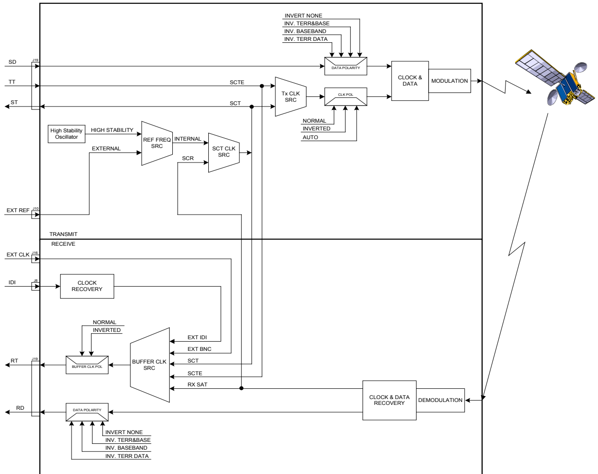
Figure 3-7 Clocking and Polarity Diagram
